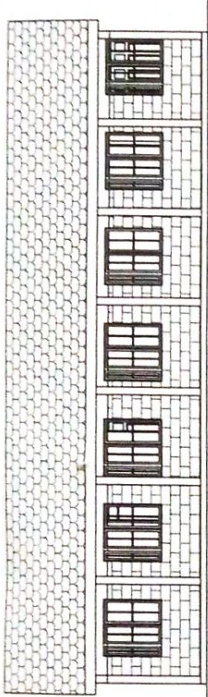
ELEVATION 03 SCALE 1:100
